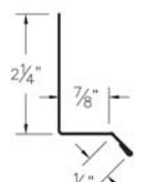
⑨ Drip Cap (DCcc)
