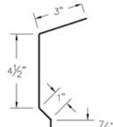
④ Fascia Trim (FTcc)
