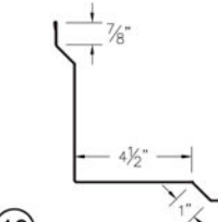
⑬ Inside Corner (ICcc)
