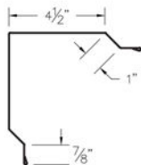
② Rake & Corner (RCcc)
