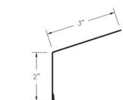
㉑ Gutter Apron (GAcc)
