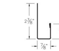
⑥ J Channel (Jcc)
