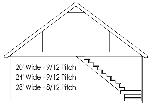
Attic Series
