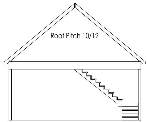
Empire Series
